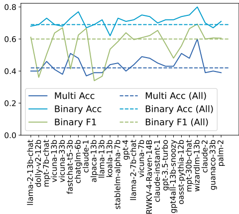
Figure 11: Predictor accuracy.
