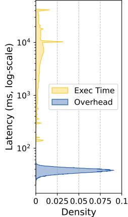
Figure 12: Overhead.
