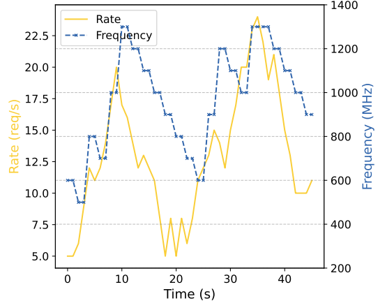
Figure 13: Frequency scaling.
