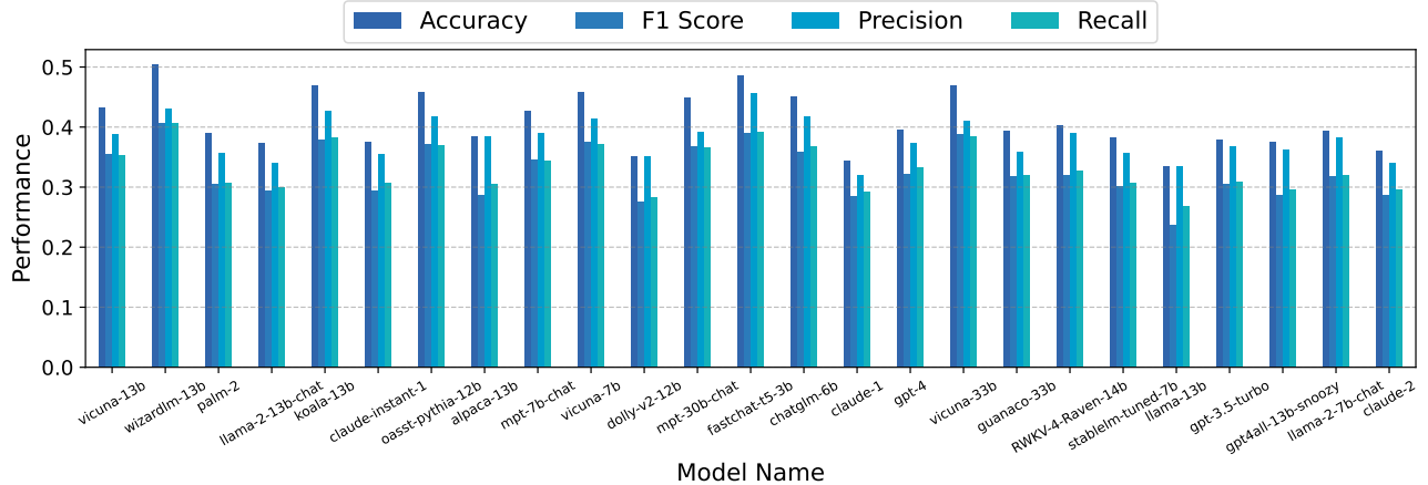
Figure 15: Output token length predictor evaluation results for each individual model.
